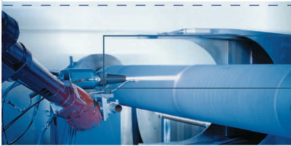
Spraying of the Rockwelle-coating
