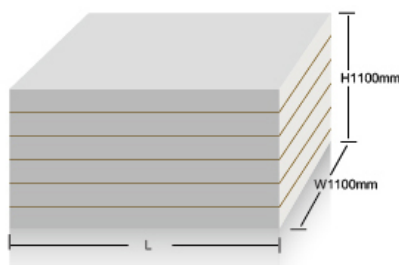
Horizontal Tying Bale size (Model XTY-1000W110110-60)
