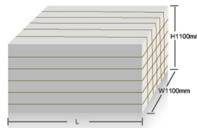
Cross Tying Bale Size (Model XTY-1000W110110-60)
