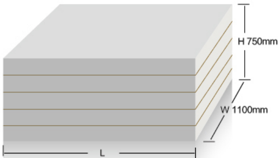
Horizontal Tying Bale size XTY-600W11075-30
