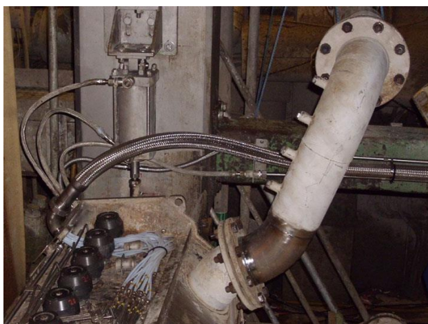
Old VIB Steambox unit replaced by a new W&H Accusteam Steambox reusing the existing control and pneumatic lifting unit
